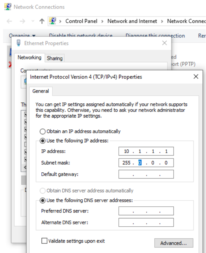
Fig. 1 — Assigning a static IP address (10.1.1.1, subnet mask 255.0.0.0) via TCP/IPv4 Properties
